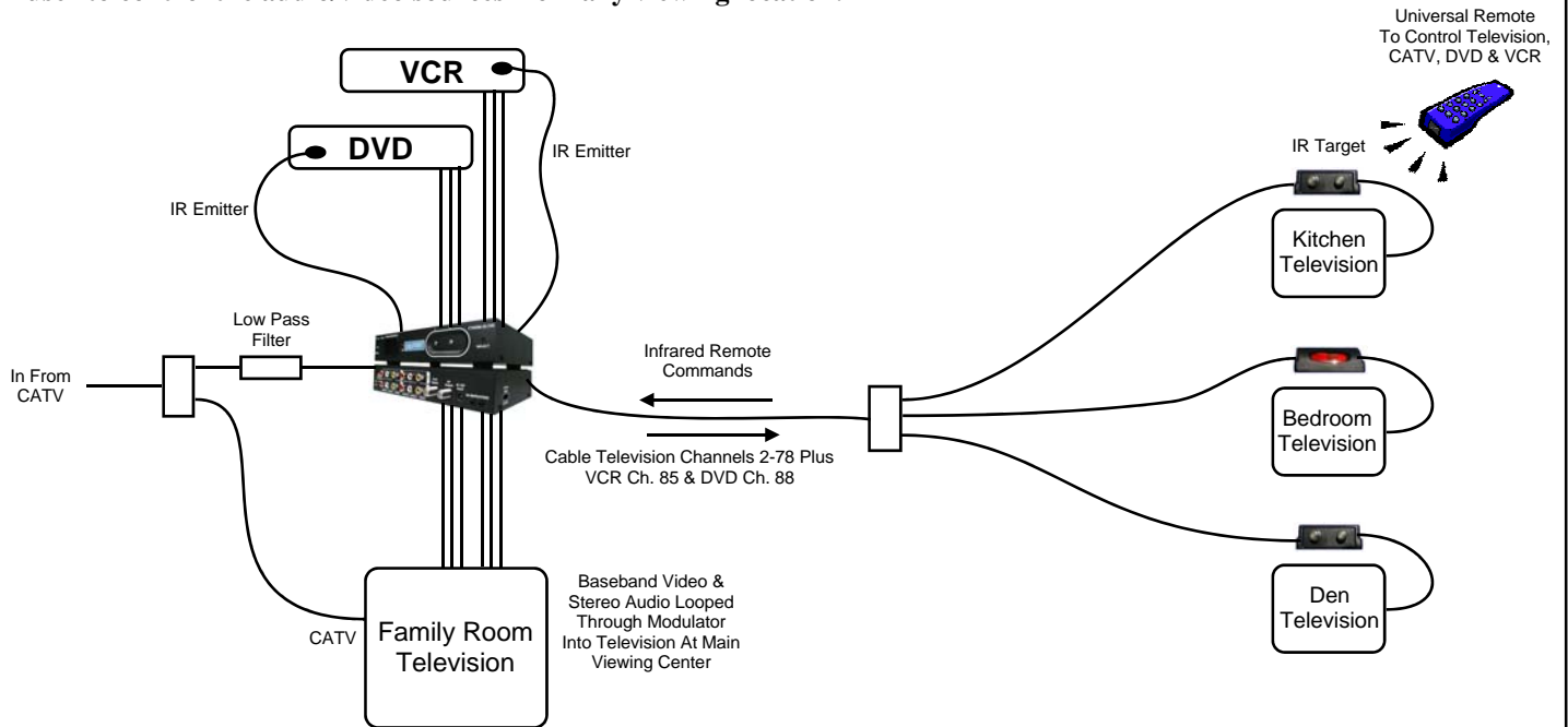
Diagram B. Two audio/video sources modulated and combined with analog cable television. Digital cable is eliminated with a low pass filter. The modulator incorporates infrared capabilities to allow the user to control the audio/video sources from any viewing location.
