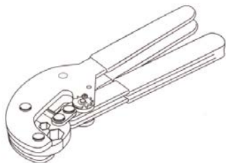
HX-596 RG-6 / RG-59 Hex Crimp Tool Crimps connectors up to .375" O.D. with up to 1/2" shank length
